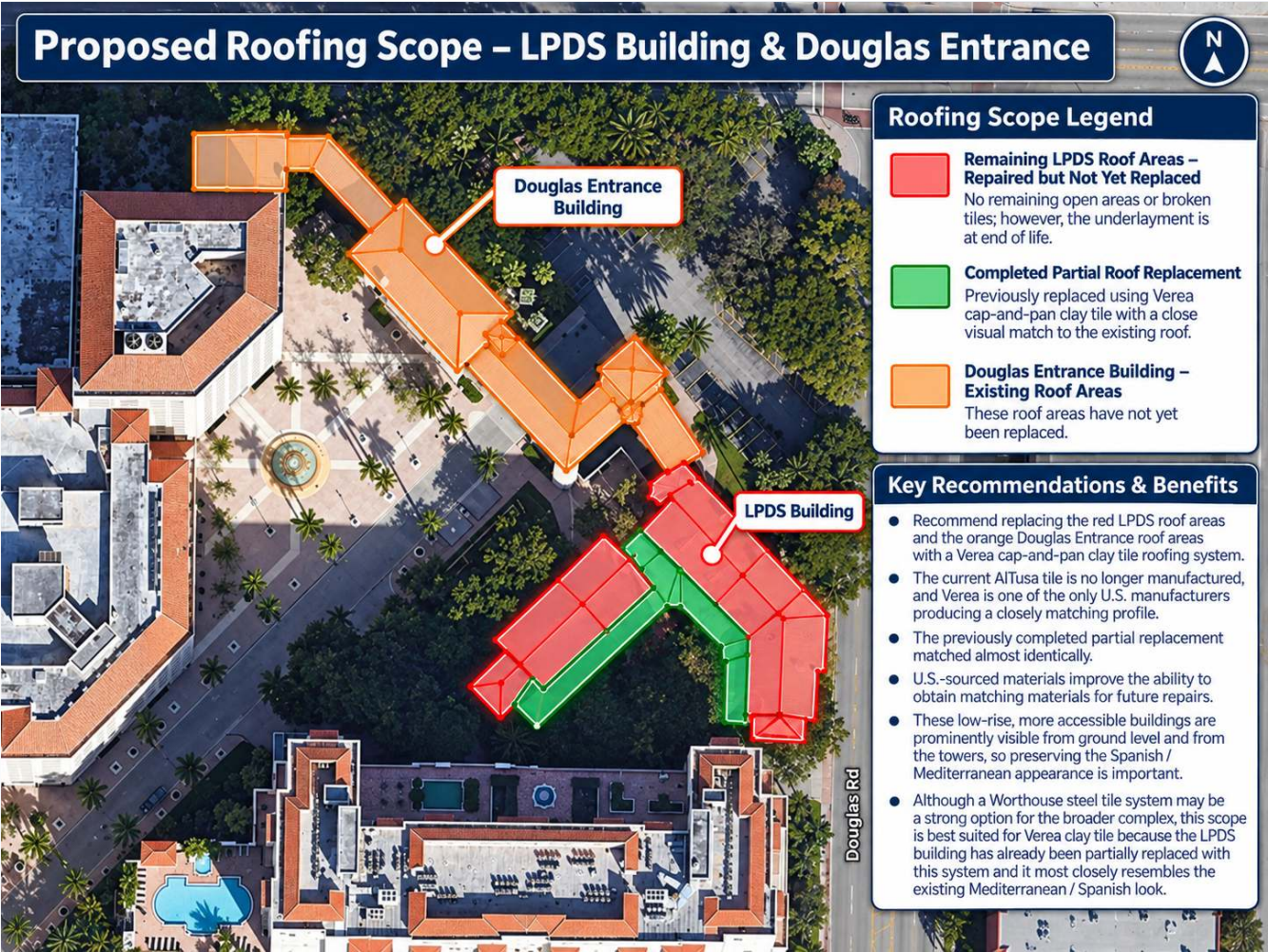
Proposed Roofing Scope — LPDS Remainder & Douglas Entrance (Verea clay). Green = completed partial Verea; orange = Douglas Entrance; red = LPDS remainder. Altusa discontinued; low-rise high-visibility → clay matches campus.
